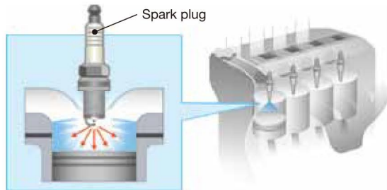
Engine's combustion chamber
